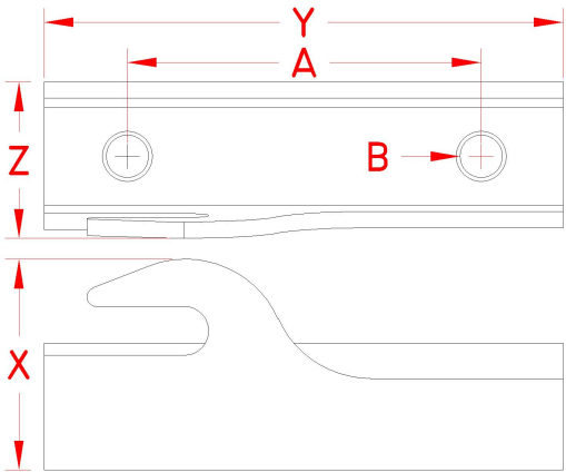
Holder drawing only; not to scale.
